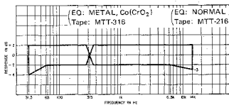
Fig. 5-5 Playback frequency response
